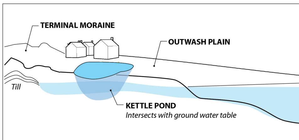
FIGURE EAW-13: Geology of Kettle Hole Ponds
