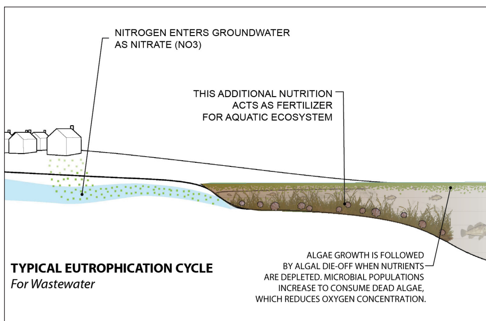
FIGURE EAW-4: The Process of Eutrophication
