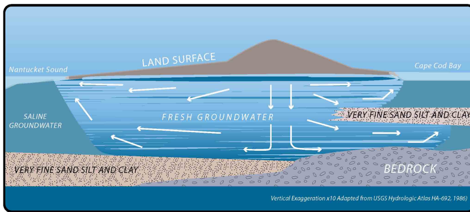
FIGURE EAW-1: Groundwater Flow Dynamics on Cape Cod
